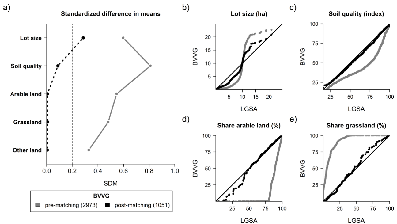
Figure D1: Matching Quality: Two-nearest neighbor matching based on Mahalanobis Distance
