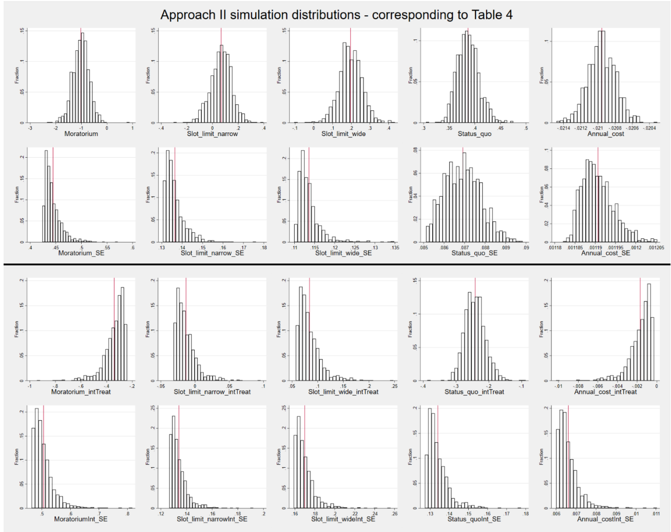
Figure E2. Distribution of estimates in the simulation of Approach II – Table 4
