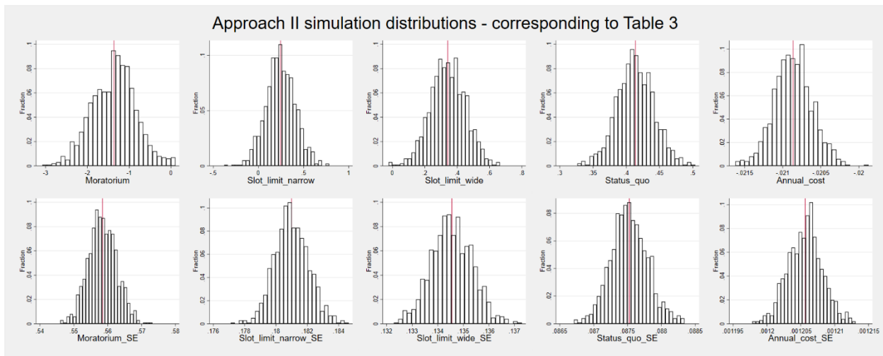
Figure E1. Distribution of estimates in the simulation of Approach II – control group in Table 3
