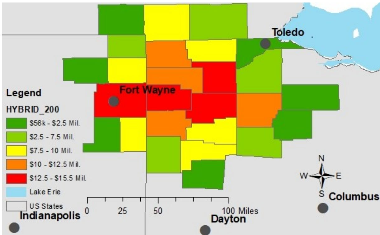
Figure E1. Policy costs and tax burden for: (a) $40/acre uniform payment, (b) $80/acre spatially targeted payment, (c) 200% tax+payment hybrid policy.
