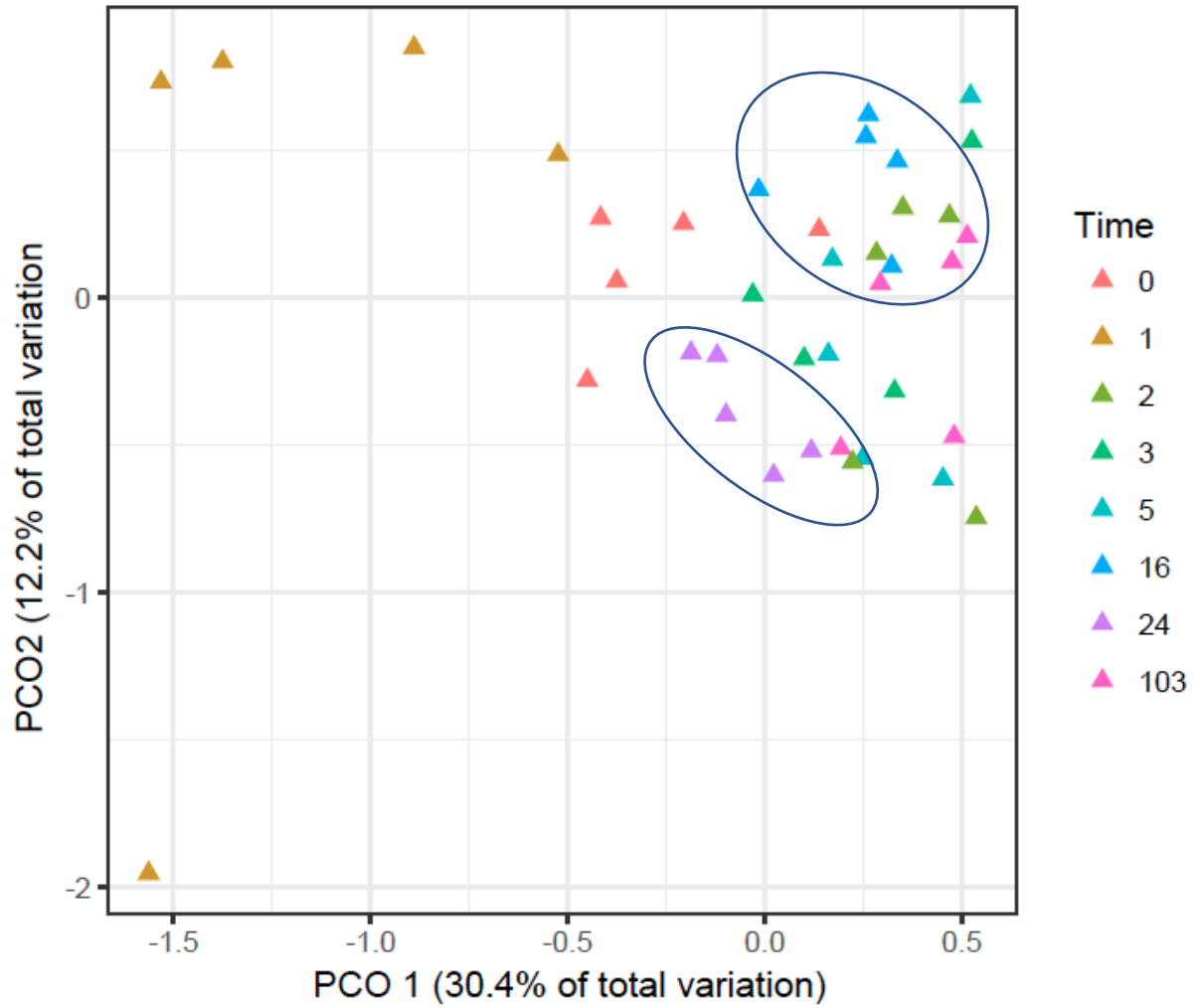
Supplemental Figure 1: Principal Coordinates analysis of AMF communities along a restoration chronosequence. Based on CSS normalized community data.
